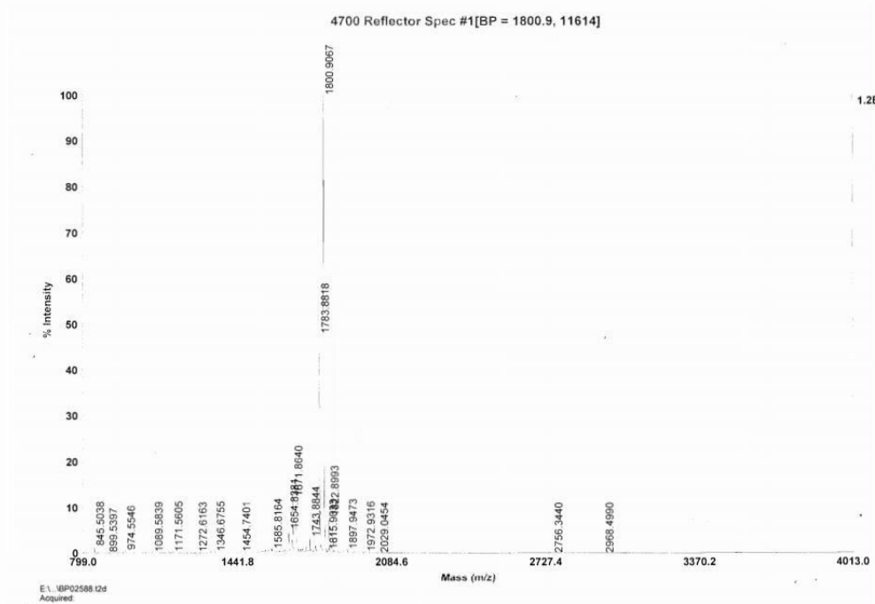
Figure 2. MASS Spectrometry
