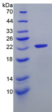
Figure 1. SDS-PAGE
