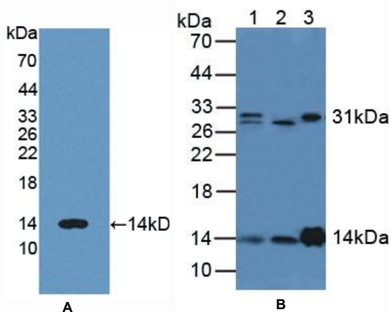
Figure 1. Western Blot
