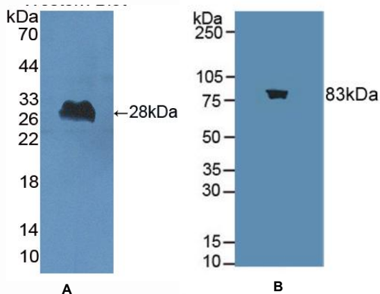
Figure 1. Western Blot
