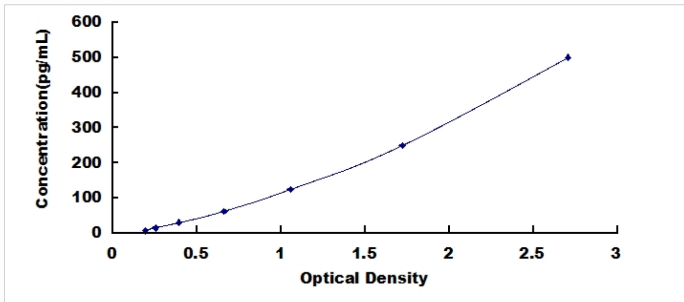
Typical Standard Curve for IL35, Mouse ELISA.
