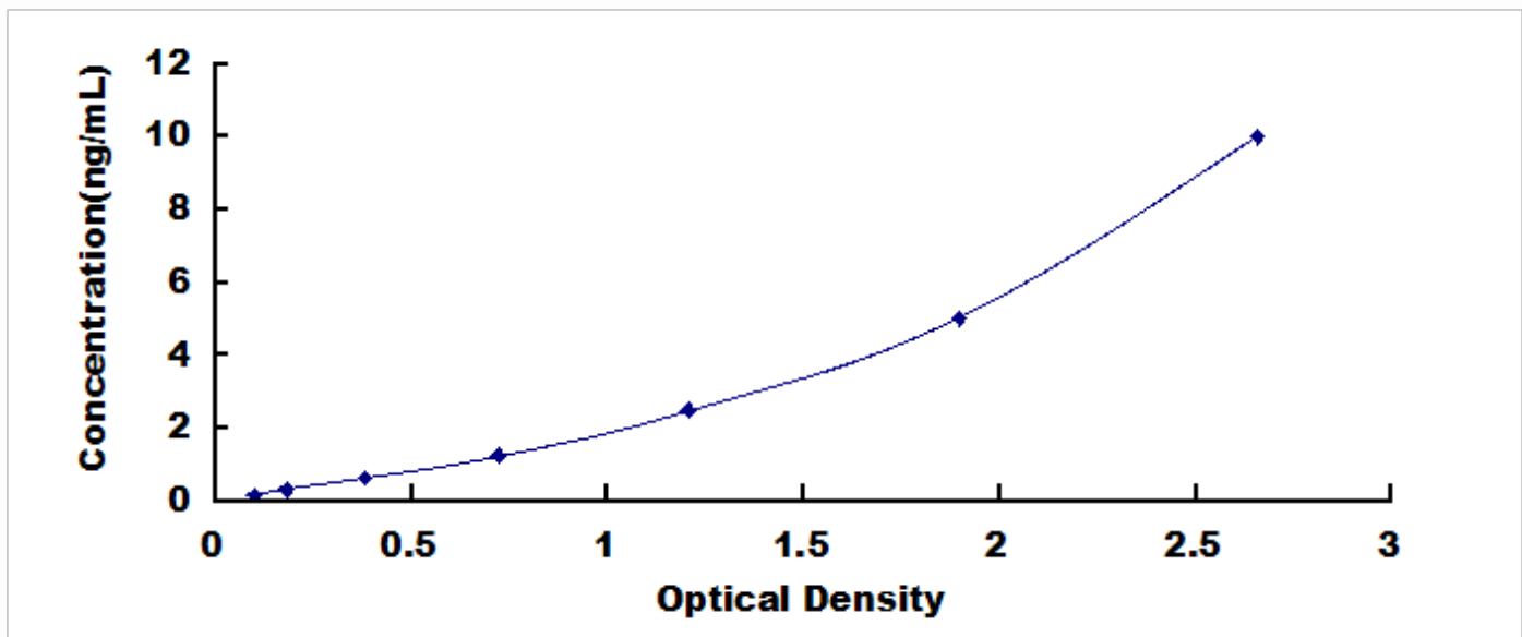
Typical Standard Curve for TLR3, Human ELISA.
