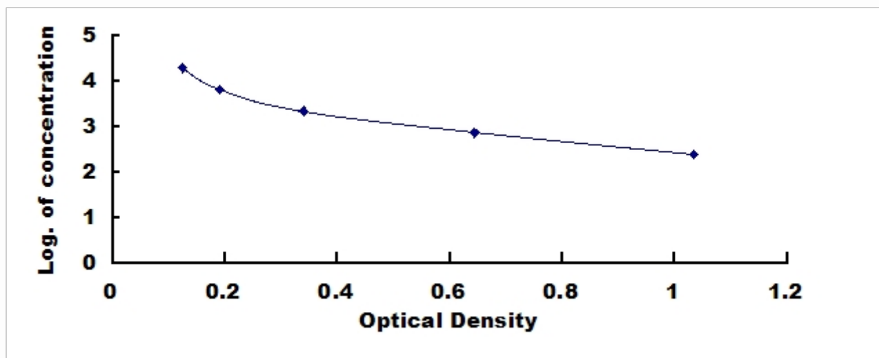
Typical Standard Curve for Sialic Acid ELISA.
