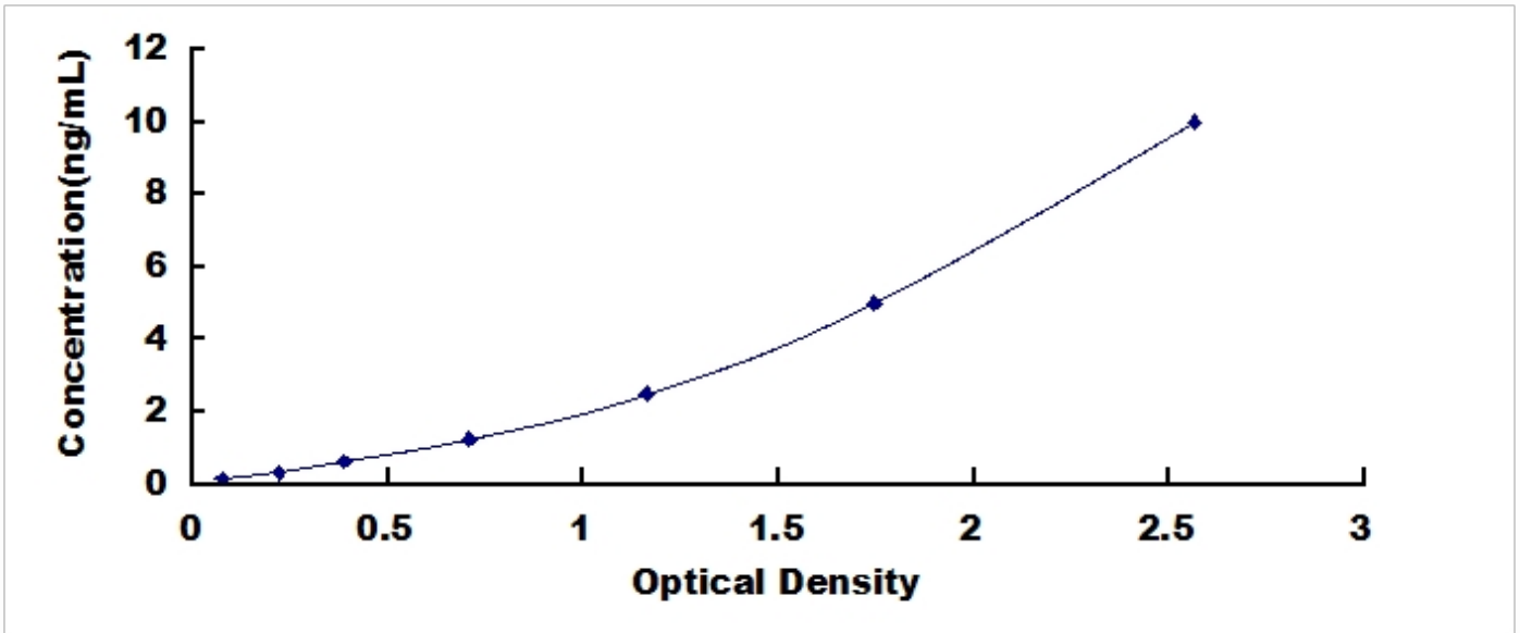
Typical Standard Curve for PR3, Mouse ELISA.
