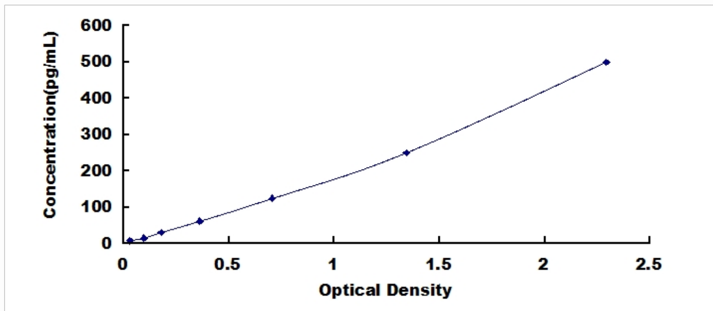
Typical Standard Curve for Pleiotrophin, Mouse ELISA.
