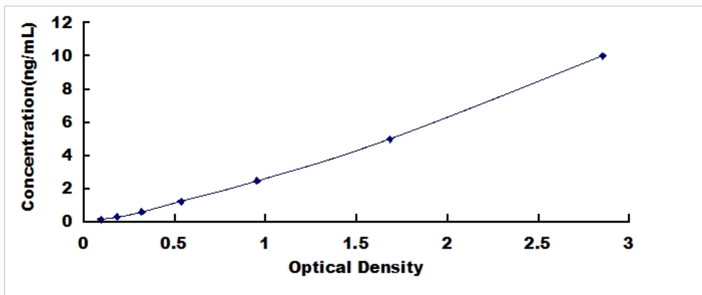
Typical Standard Curve for Noggin, Mouse ELISA.
