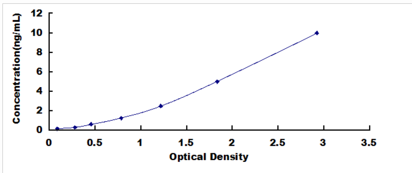
Typical Standard Curve for MBL, Mouse ELISA.
