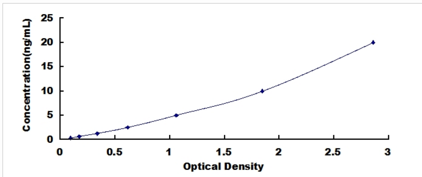
Typical Standard Curve for MIF, Human ELISA.
