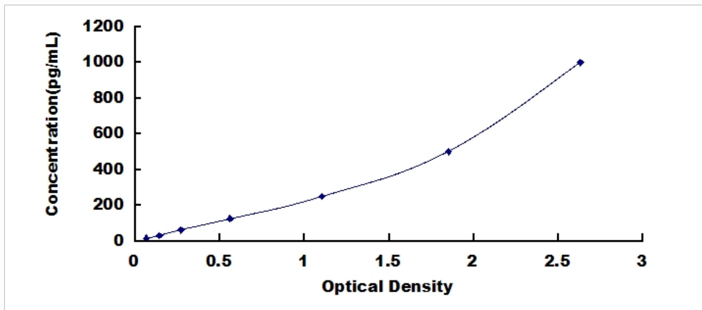
Typical Standard Curve for IL4, Human ELISA.
