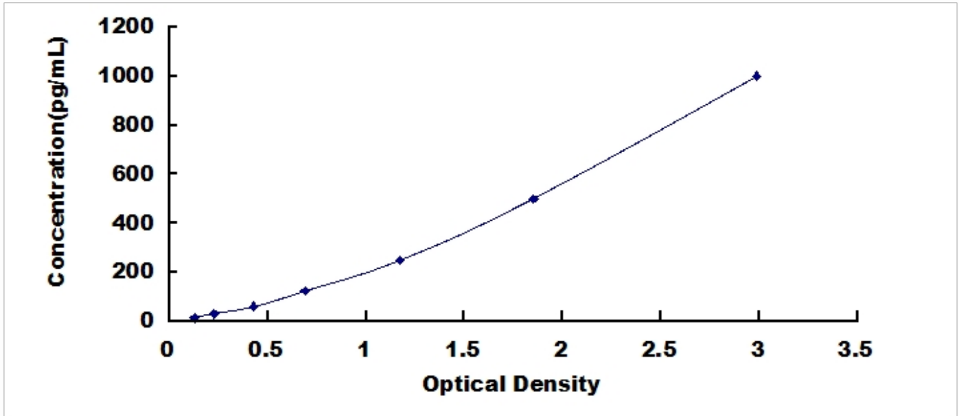
Typical Standard Curve for IL10, Rabbit ELISA.
