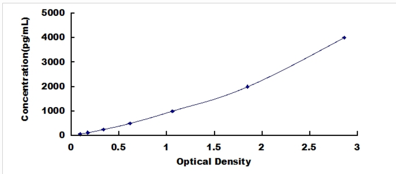
Typical Standard Curve for Hepcidin, Human ELISA.
