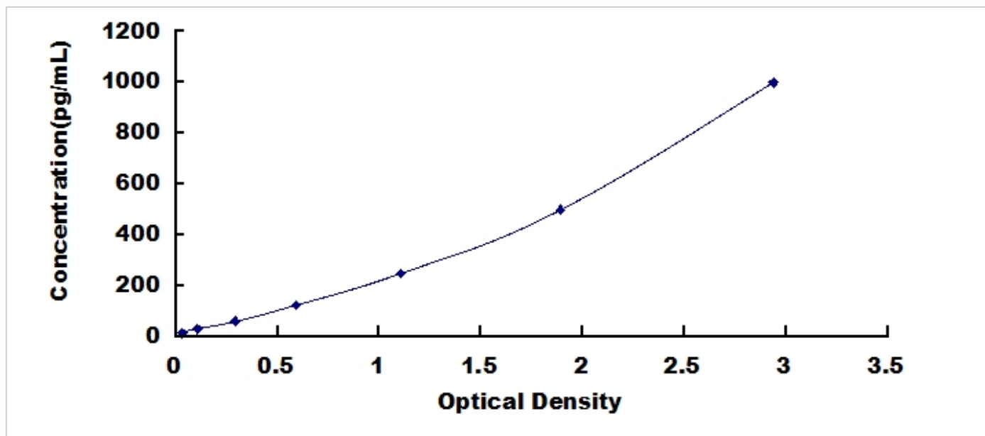
Typical Standard Curve for FGF23, Human ELISA.
