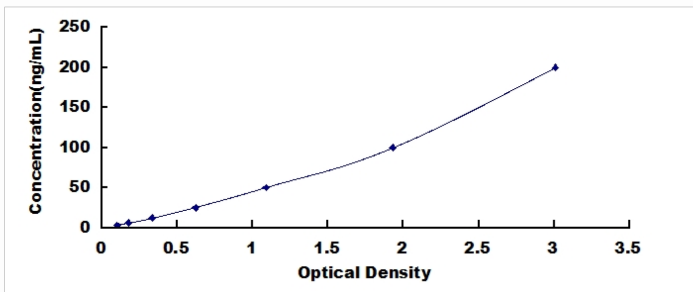
Typical Standard Curve for Anti-TG, Human ELISA.
