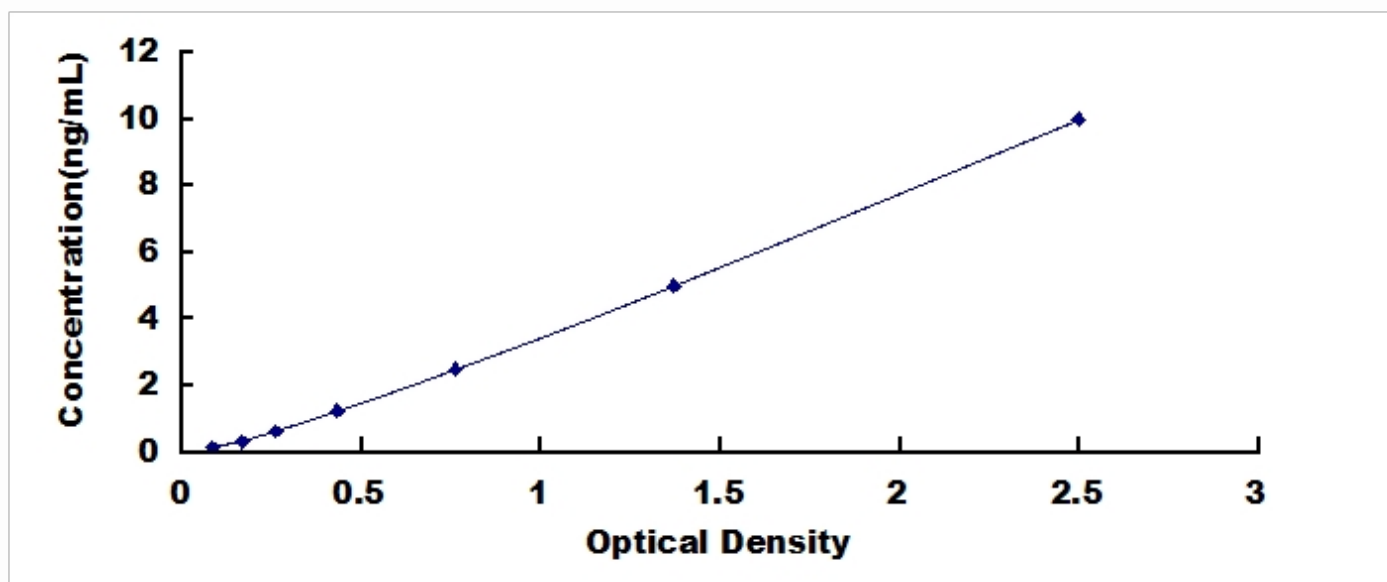
Typical Standard Curve for ANGPTL2, Rat ELISA.
