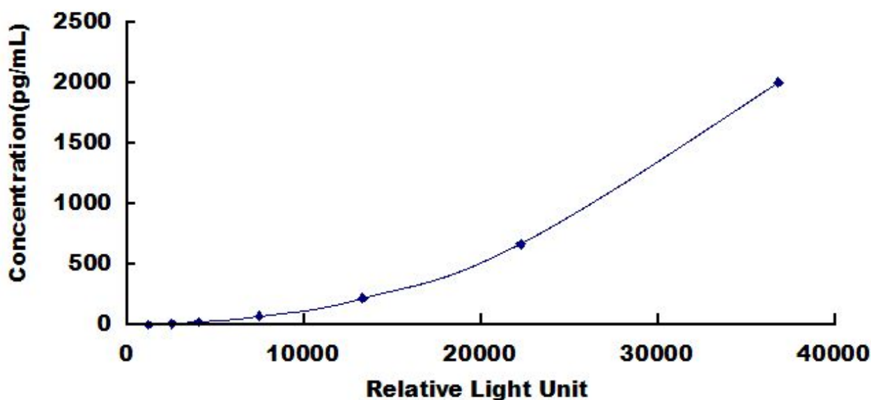
Typical Standard Curve for EBI3, Human CLIA.
