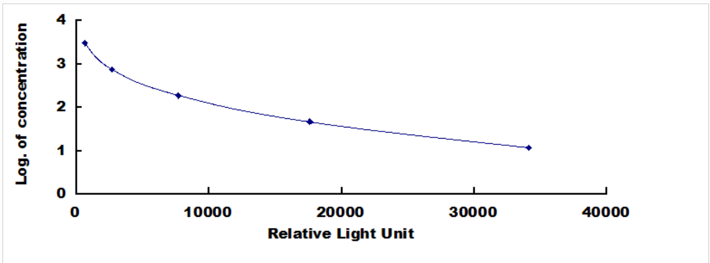
Typical Standard Curve for Dopamine CLIA.
