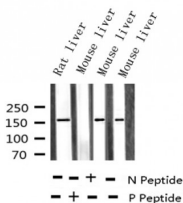
Western blot analysis of Phospho-EGFR (Tyr1110) expression in various lysates
