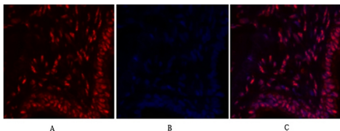
Fig.2. Immunofluorescence analysis of human lung tissue. 1, c-Myc Polyclonal Antibody (red) was diluted at 1:200 (4°C, overnight). 2, Cy3 labeled secondary antibody was diluted at 1:300 (room temperature, 50min). 3, Picture B: DAPI (blue) 10min. Picture A: Target. Picture B: DAPI. Picture C: merge of A+B.
